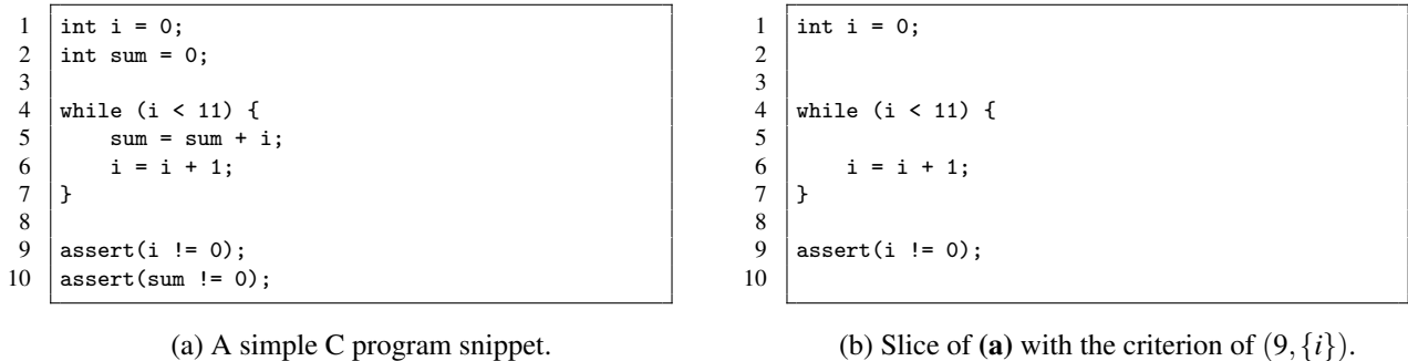
Figure 1: A slicing example.
