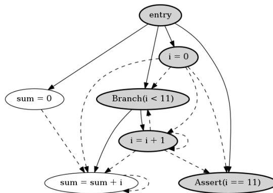
Figure 2: Slicing on the assert node using a program dependence graph.
