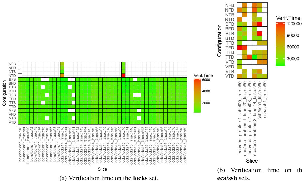
Figure 10: Heat map of verification time for slices with different configurations.
