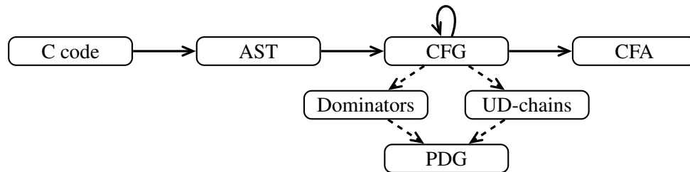
Figure 4: Transformation workflow.
