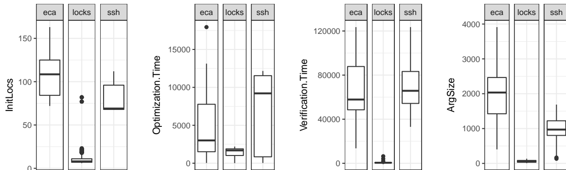
Figure 6: Overview of output variables.
